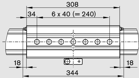
Carriage with clamping unit and air ports
