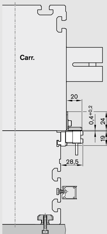
Proximity switches with mounting accessories / cable duct
