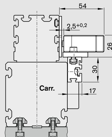
Mechanical switches with mounting accessories
