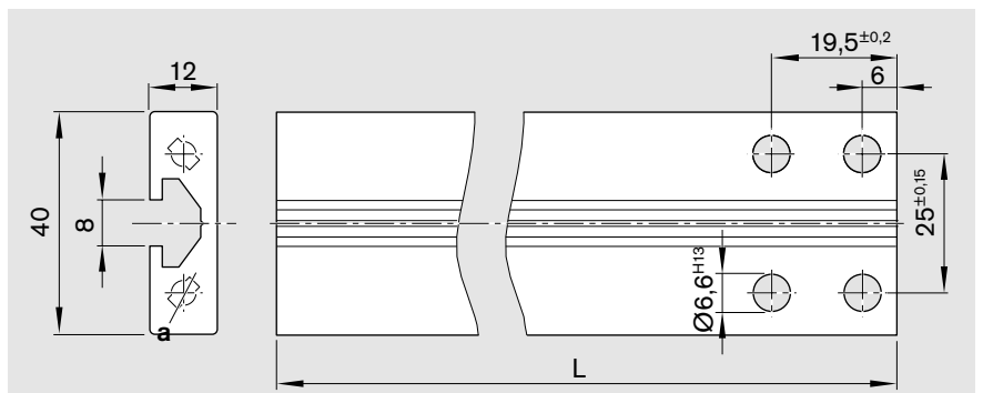
a) For M5 self-tapping screws
