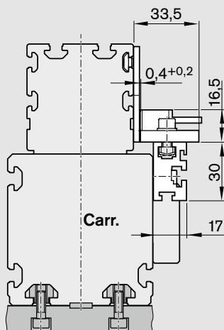
Proximity switches with mounting accessories
