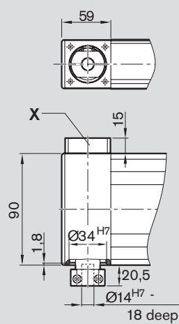
Types MA05 and MA06
