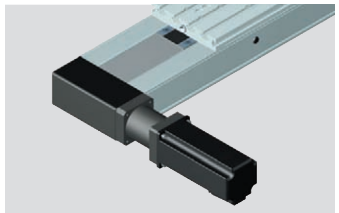
Gear reducer: A variety of gear ratios allow an optimal match between the load and the drive motor inertia.
