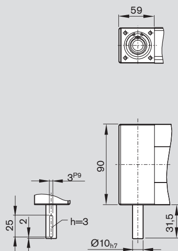
Types MA01 and MA02
