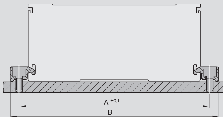
Mounting with clamping fixtures
