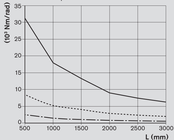
Torsional stiffness c_T
