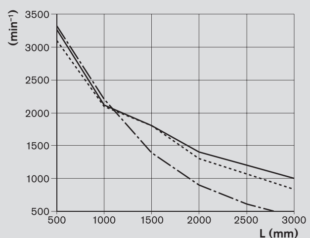
Maximum rotary speed n
