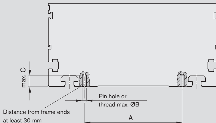
Special modification in the base surface of the frame (not from factory)
