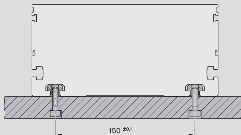
Special modification in the base surface of the frame (not from factory)
